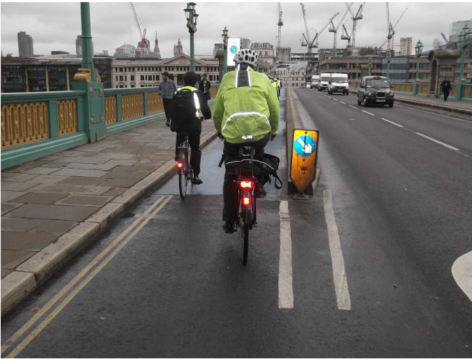
Southwark Bridge, London. The start of a run of containment kerbs protecting the bridge parapet, but providing a cycle track too (containment kerbs behind the keep right sign).
