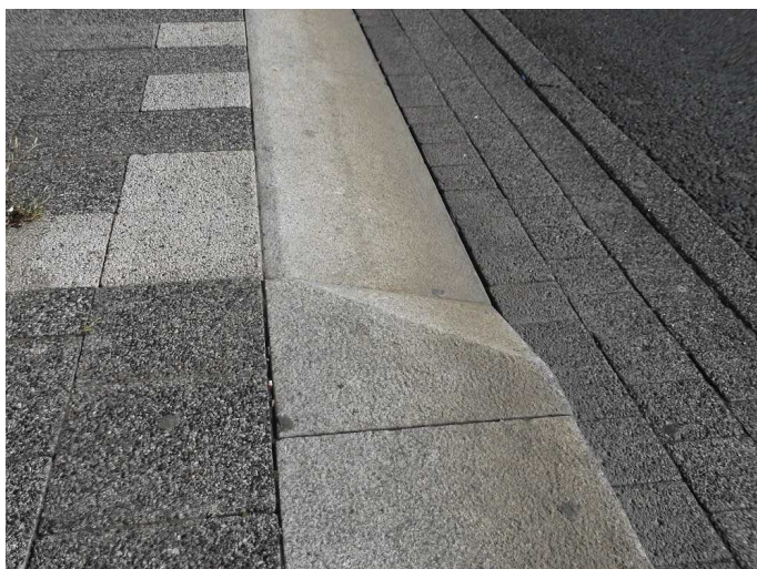
Machined and textured granite transition and ramp kerb.
