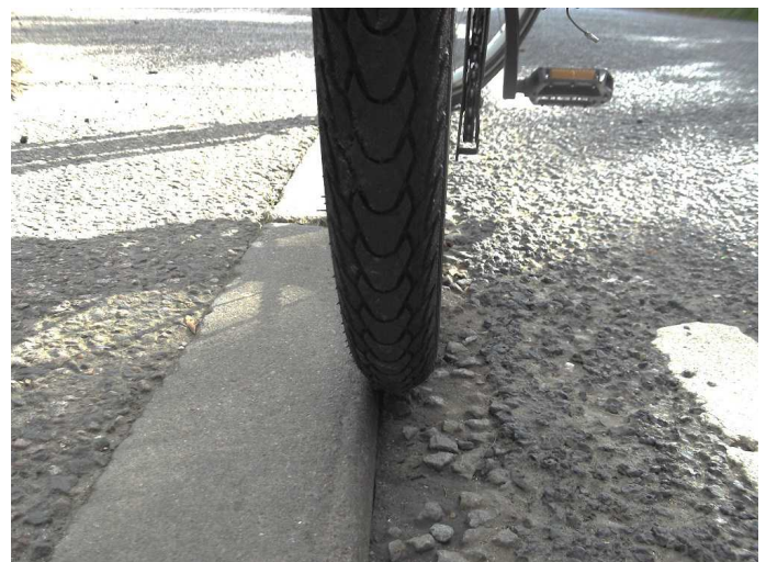
A kerb upstand will “grab” the wheels and throw the rider off their cycle.
