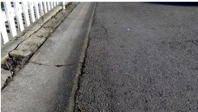
Dished channel at rear of footway to stop water running onto private land behind.
